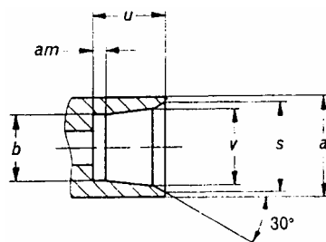
Figure 8 – Gauge for outer contact of pin connector
