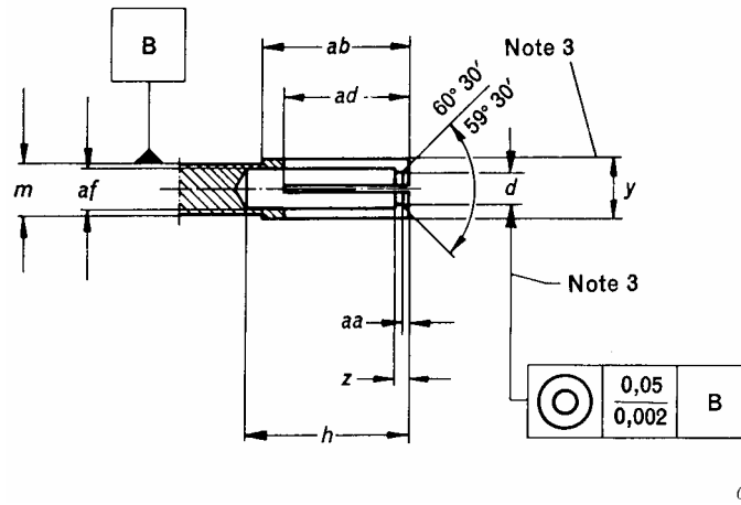
Figure 14 – Dimensions of centre contact (see Table 7)
